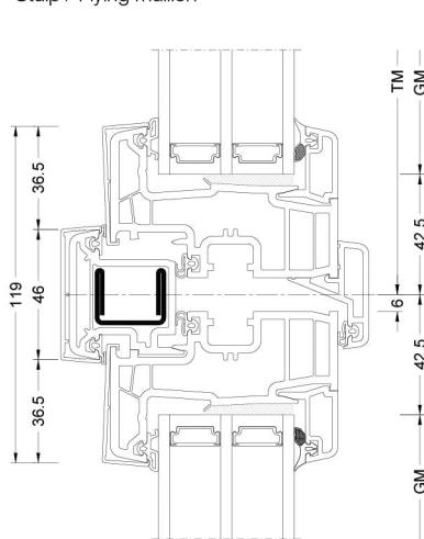
Stulp / Flying mullion
