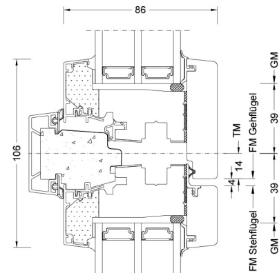
Stulp / Flying mullion
